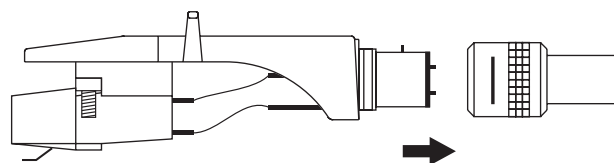
Figure 5 – Headshell
